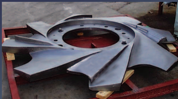
Pulper Impeller for use in Recycle Area, "High Wear"
