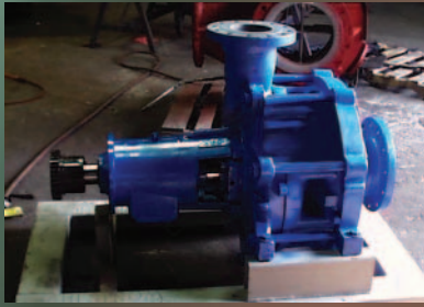
Ahlstrom LRS Pump. Use: 4-6 pumps for every digester. ProCast Makes all Parts.
