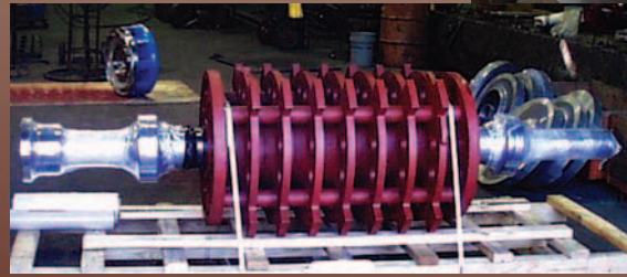
Screen Rotor for Use in Pulp Mill "Repair or New"
