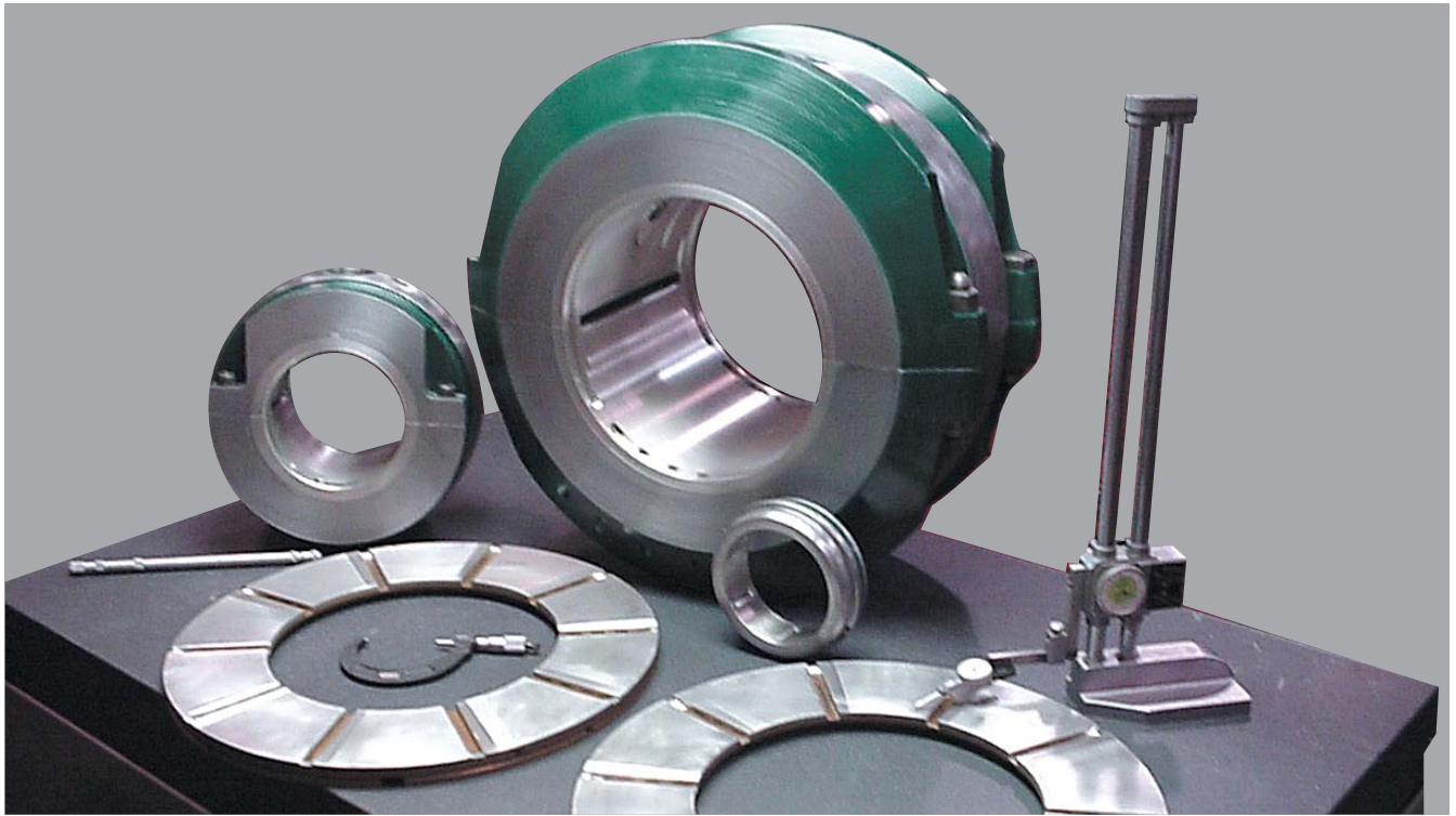
Large steam turbine bearings re-Babbitted per OEM specifications.
