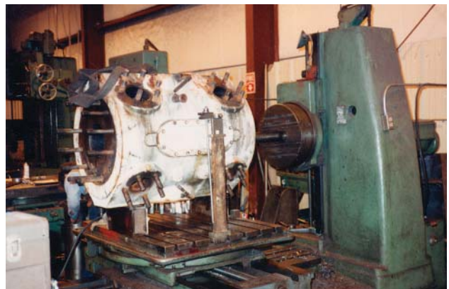
Cylinder being bored to accept new liner.
