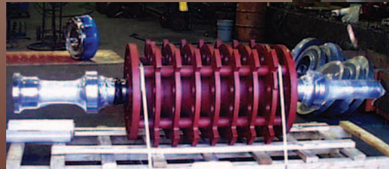
Screen Rotor for Use in Pulp Mill "Repair or New"
